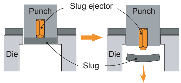
Fig.1 Pushing slug mechanism by slug ejector
