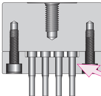
Fig.5 Cluster tooling
